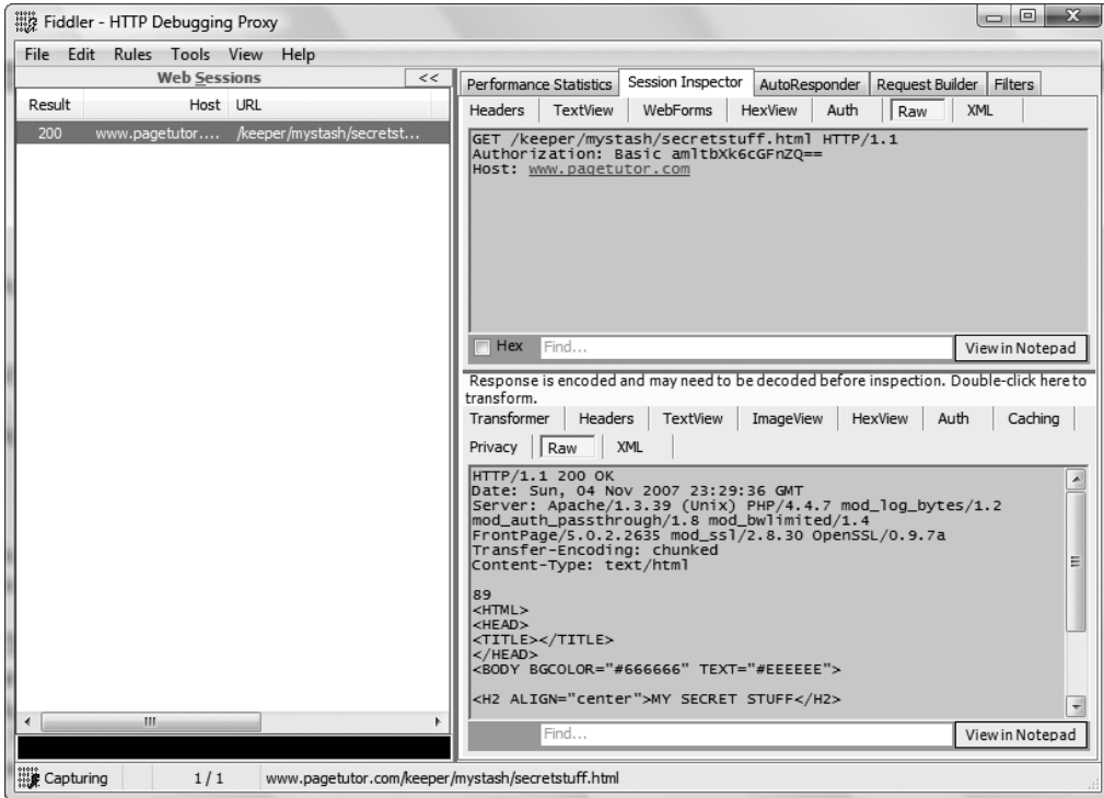
Figure 17-6. Fiddler showing a request to a password-protected page
